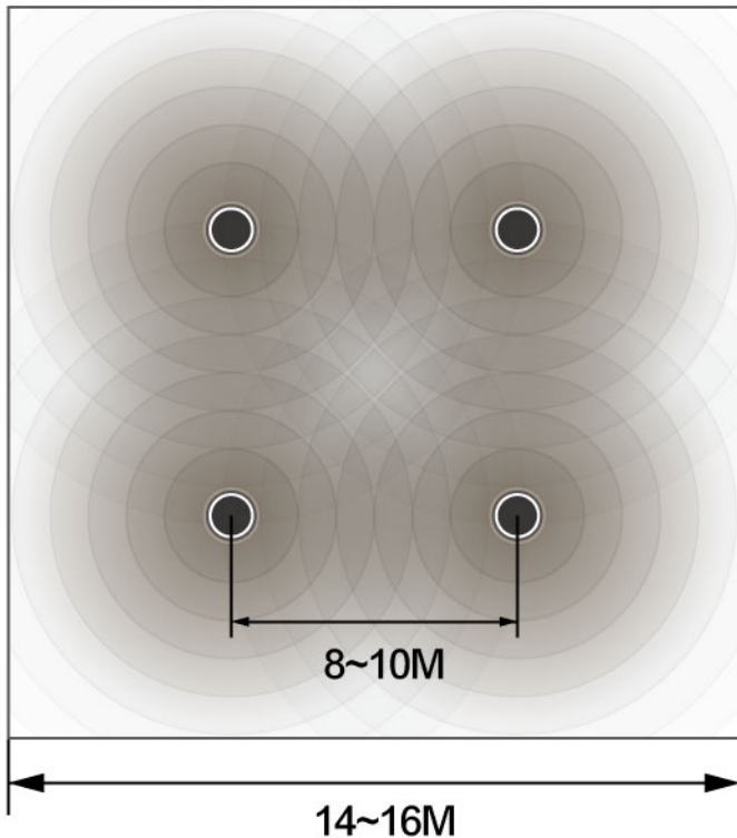
Traditional ceiling speaker arrangement and its coverage
